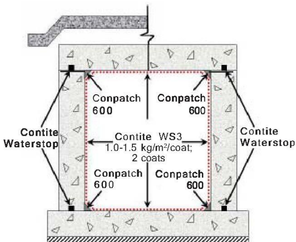
Closed Water Retaining Structure Waterproofing
